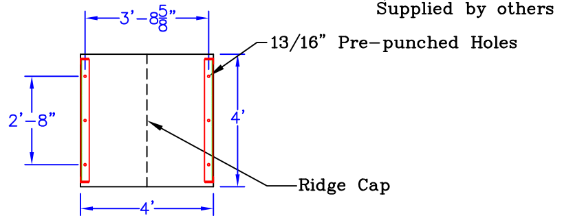
Mounting Detail
