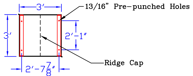
Mounting Detail
