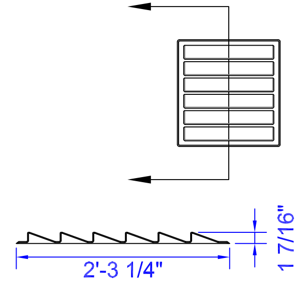
Cross-Section Side View
