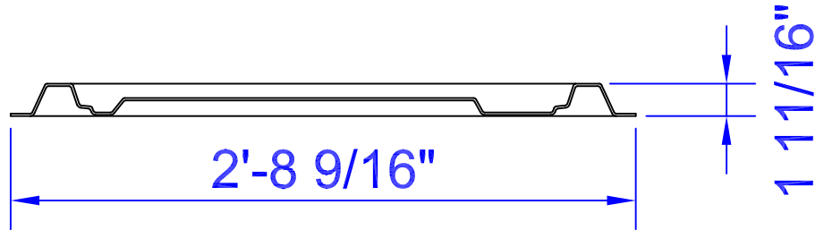
Cross-Section Side View
